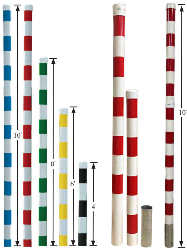
10' and 8' yardage poles come in 2 pieces. Shown beside 12" Steel ground anchor
